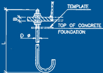
ANCHOR BOLT - 'J' TYPE 'L' TYPE ANCHOR BOLT CAN BE PROVIDED AS PER CLIENT'S REQUIREMENT
